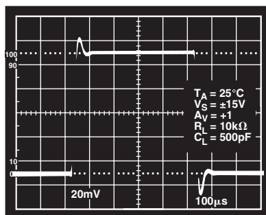
TPC 14. Small-Signal Transient Response
