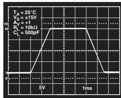
TPC 15. Large-Signal Transient Response
